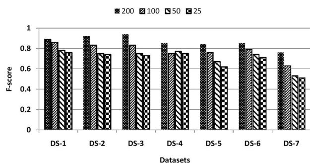
Fig. 6 Effect of different GloVe embeddings dimensions (200, 100, 50, and 25) on the classification results of CAT-BiGRU model over Ptáček et al. [30] (DS-1), SemEval 2015 [4] (DS-2), Riloff et al. [22] (DS-3), Bamman and Smith [32] (DS-4), Ghosh and Veale [33] (DS-5), Ling and Klinger [31] (DS-6), and Twitter-280 (DS-7) datasets in terms of f-score
