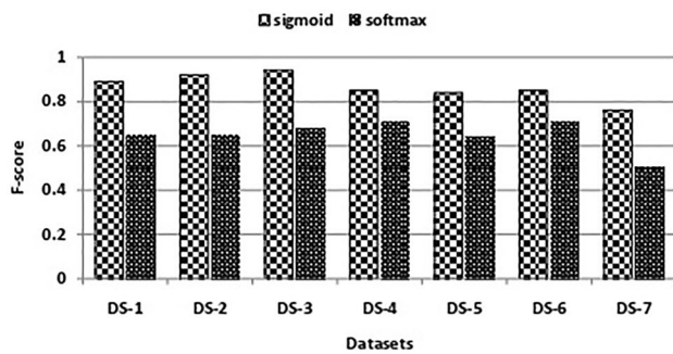
Fig. 12 Effect of different activation functions ( sigmoid and softmax ) on the classification results of CAT-BiGRU model over Ptáček et al. [30] (DS-1), SemEval 2015 [4] (DS-2), Riloff et al. [22] (DS-3), Bamman and Smith [32] (DS-4), Ghosh and Veale [33] (DS-5), Ling and Klinger [31] (DS-6), and Twitter-280 (DS-7) datasets in terms of f-score
