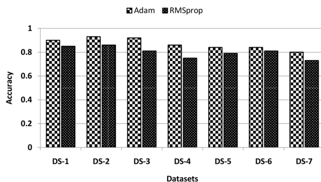
Fig. 11 Effect of different optimization algorithms ( Adam and RMSprop ) on the classification results of CAT-BiGRU model over Ptáček et al. [30] (DS-1), SemEval 2015 [4] (DS-2), Riloff et al. [22] (DS-3), Bamman and Smith [32] (DS-4), Ghosh and Veale [33] (DS-5), Ling and Klinger [31] (DS-6), and Twitter-280 (DS-7) datasets in terms of accuracy
