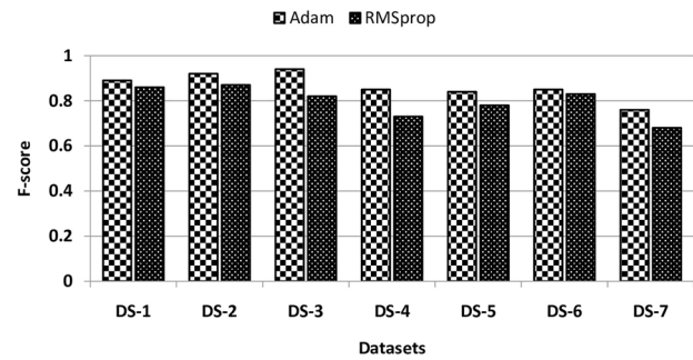
Fig. 10 Effect of different optimization algorithms ( Adam and RMSprop ) on the classification results of CAT-BiGRU model over Ptáček et al. [30] (DS-1), SemEval 2015 [4] (DS-2), Riloff et al. [22] (DS-3), Bamman and Smith [32] (DS-4), Ghosh and Veale [33] (DS-5), Ling and Klinger [31] (DS-6), and Twitter-280 (DS-7) datasets in terms of f-score
