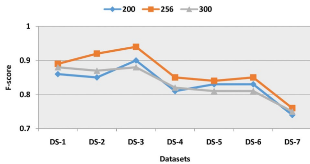
Fig. 8 Effect of different GRU hidden units (200, 256, and 300) on the classification results of CAT-BiGRU model over Ptáček et al. [30] (DS-1), SemEval 2015 [4] (DS-2), Riloff et al. [22] (DS-3), Bamman and Smith [32] (DS-4), Ghosh and Veale [33] (DS-5), Ling and Klinger [31] (DS-6), and Twitter-280 (DS-7) datasets in terms of f-score
