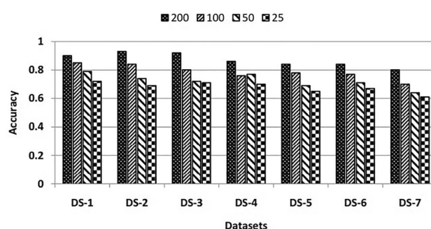
Fig. 7 Effect of different GloVe embeddings dimensions (200, 100, 50, and 25) on the classification results of CAT-BiGRU model over Ptáček et al. [30] (DS-1), SemEval 2015 [4] (DS-2), Riloff et al. [22] (DS-3), Bamman and Smith [32] (DS-4), Ghosh and Veale [33] (DS-5), Ling and Klinger [31] (DS-6), and Twitter-280 (DS-7) datasets in terms of accuracy
