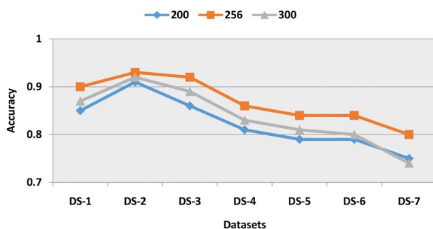
Fig. 9 Effect of different GRU hidden units (200, 256, and 300) on the classification results of CAT-BiGRU model over Ptáček et al. [30] (DS-1), SemEval 2015 [4] (DS-2), Riloff et al. [22] (DS-3), Bamman and Smith [32] (DS-4), Ghosh and Veale [33] (DS-5), Ling and Klinger [31] (DS-6), and Twitter-280 (DS-7) datasets in terms of accuracy
