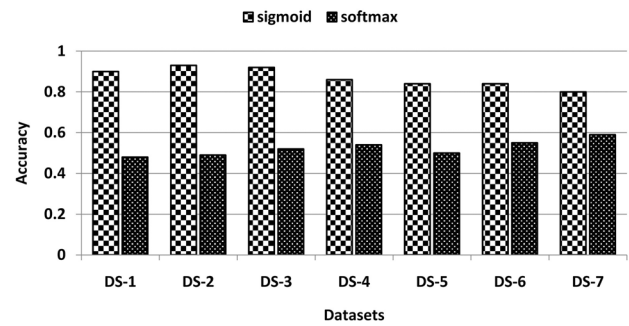
Fig. 13 Effect of different activation functions ( sigmoid and softmax ) on the classification results of CAT-BiGRU model over Ptáček et al. [30] (DS-1), SemEval 2015 [4] (DS-2), Riloff et al. [22] (DS-3), Bamman and Smith [32] (DS-4), Ghosh and Veale [33] (DS-5), Ling and Klinger [31] (DS-6), and Twitter-280 (DS-7) datasets in terms of accuracy
